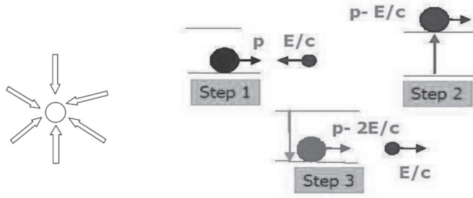
Figure 2. (a) Schematic diagram of Laser cooling technique
