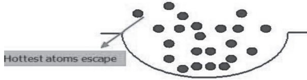
Figure 3. Schematic diagram of the evaporative cooling
