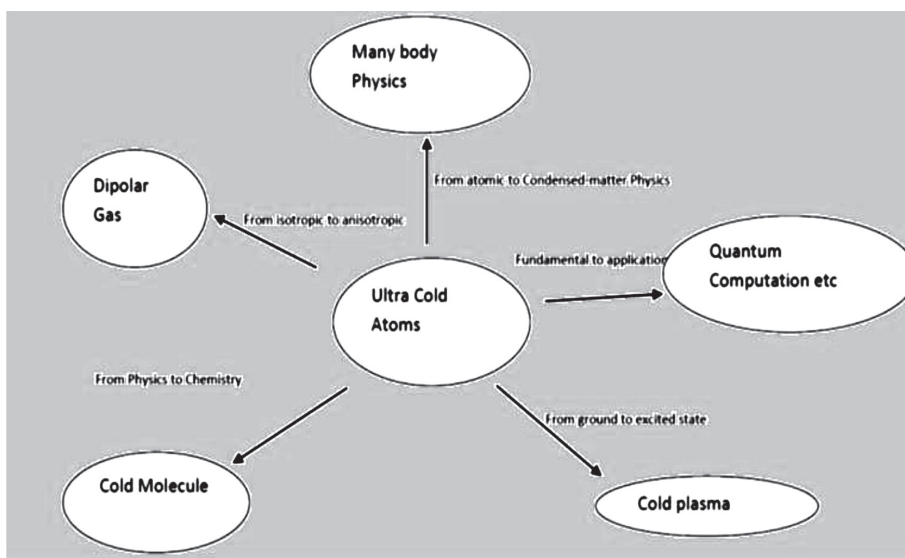
Figure 1. Schematic diagram of different fields of Ultra-cold research
